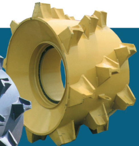
CAT 826 C/G High Density Wheel
